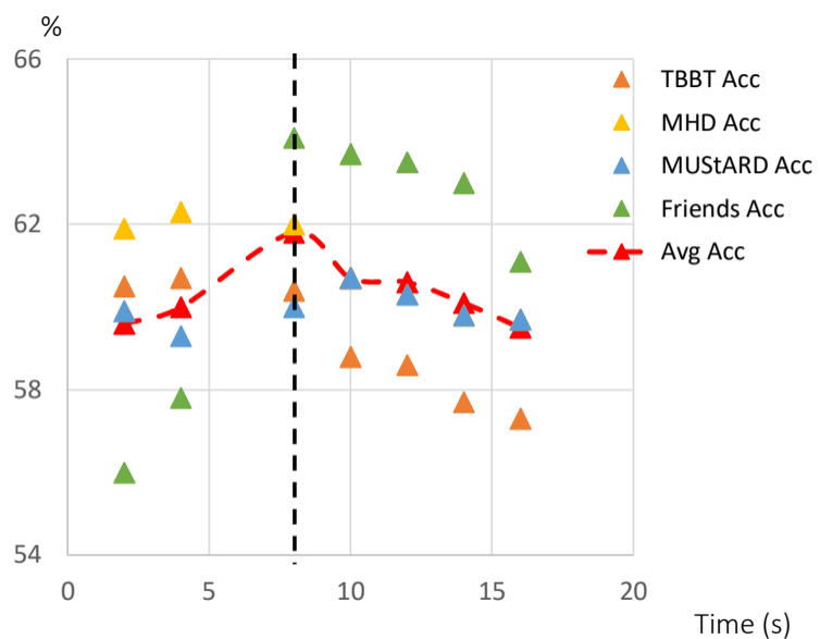
(b) FunnyNet-W V: Accuracy VS Time windows
