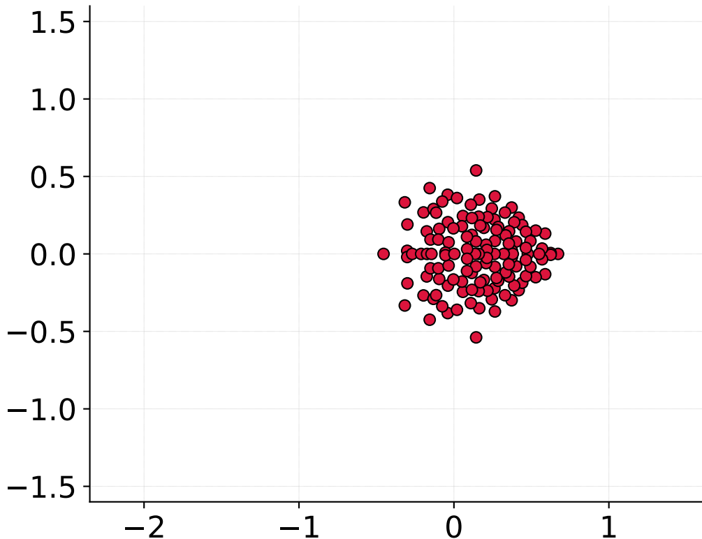
Eigenvalues of value matrix for head 14
