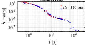
Hexadecane
