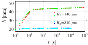
Hexadecane
