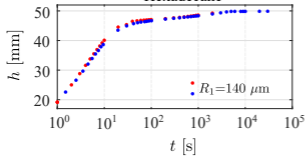
Hexadecane
